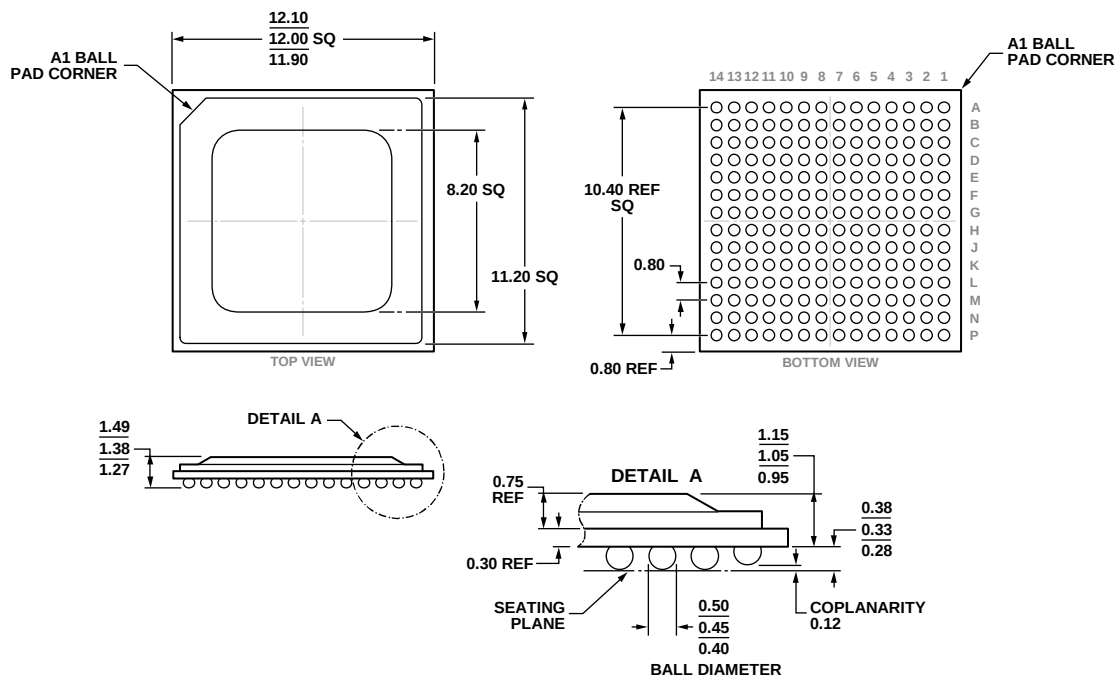
Figure 71. 196-Ball Ball Grid Array, Thermally Enhanced [BGA_ED] (BP-196-3)
