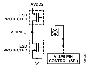
Figure 38. V_1P0 Input/Output
